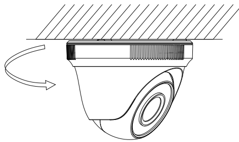
Figure 2. 11 Secure the Camera with Mounting Base
