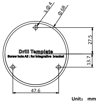
Figure 2. 1 Drill Template
