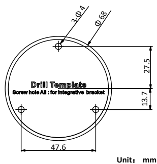
Figure 2. 5 Drill Template
