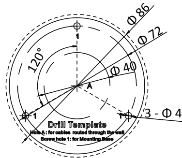
Figure 2. 9 Drill Template
