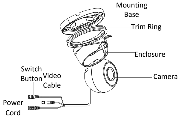
Figure 1. 2 Type II Camera Overview
