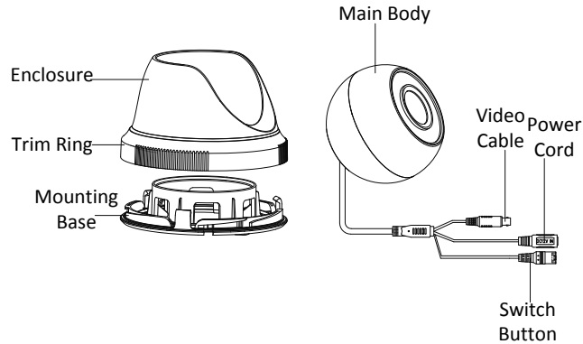
Figure 1. 3 Type III Camera Overview
