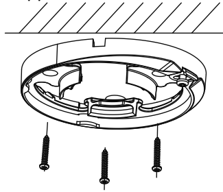
Figure 2. 6 Attach the Mounting Base to the Ceiling
