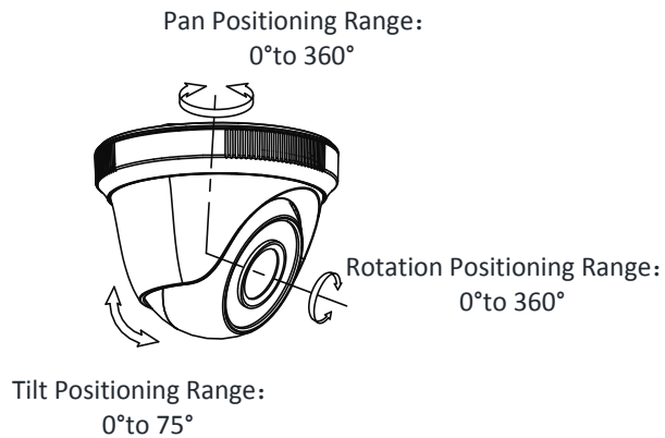
Figure 2. 12 3-axis Adjustment
