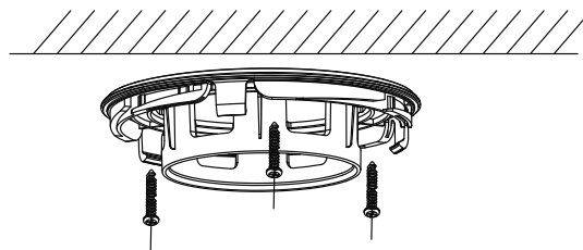
Figure 2. 10 Attach the Mounting Base to the Ceiling
