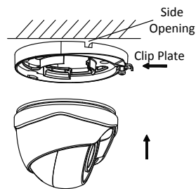
Figure 2. 7 Secure the Camera with Mounting Base
