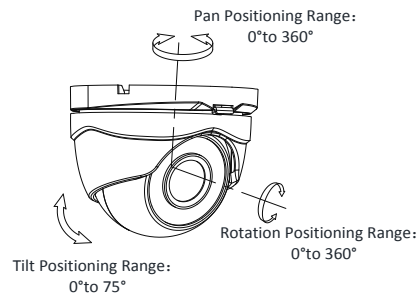
Figure 2. 8 3-axis Adjustment
