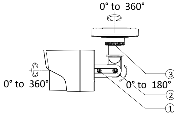
Figure 2. 3 3-Axis Adjustment
